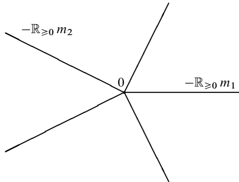
Figure 1: Tropicalization of \bar{Y}_m .
