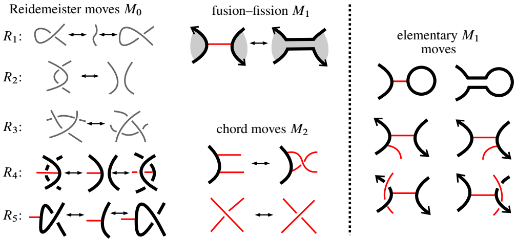
Figure 11: Kawauchi’s M_0 , M_1 and M_2 moves for chord diagrams in S^4 . In moves R_4, R_5, M_1 and M_2 the red (narrow) curves represent \alpha arcs, while black (bold) curves represent components of o . The (gray) curves of moves R_1, R_2 and R_3 represent arcs from either \alpha or o .
