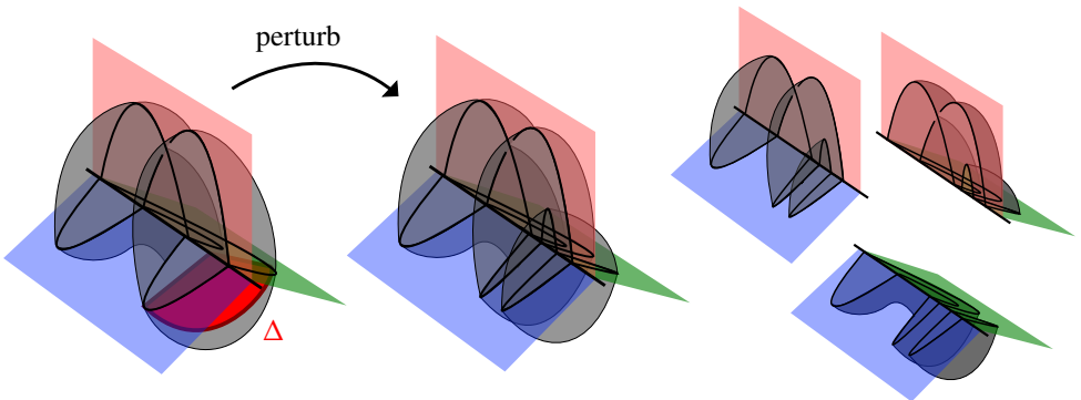
Figure 8: Left: \Sigma \cong \mathbb{R}P^2 in (1, 1, 1; 2) -bridge position in S^4 (with respect to the standard trisection). We indicate a disk \Delta along which we perturb. Right: after perturbing, \Sigma is in (1, 2, 1; 3) -bridge position (up to permuting X_1, X_2 and X_3 ).
