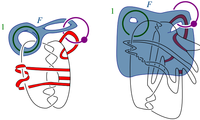
Figure 9: Left: a banded unlink for a torus in \mathbb{C}P^2\#(S^1 \times S^3) . The surface F induces a genus-2 Heegaard splitting H \cup_F H' on M_1 = S^1 \times S^2 . Right: we isotope the banded unlink into bridge position with respect to the Heegaard splitting H \cup_F H' , as in Definition 5.11.
