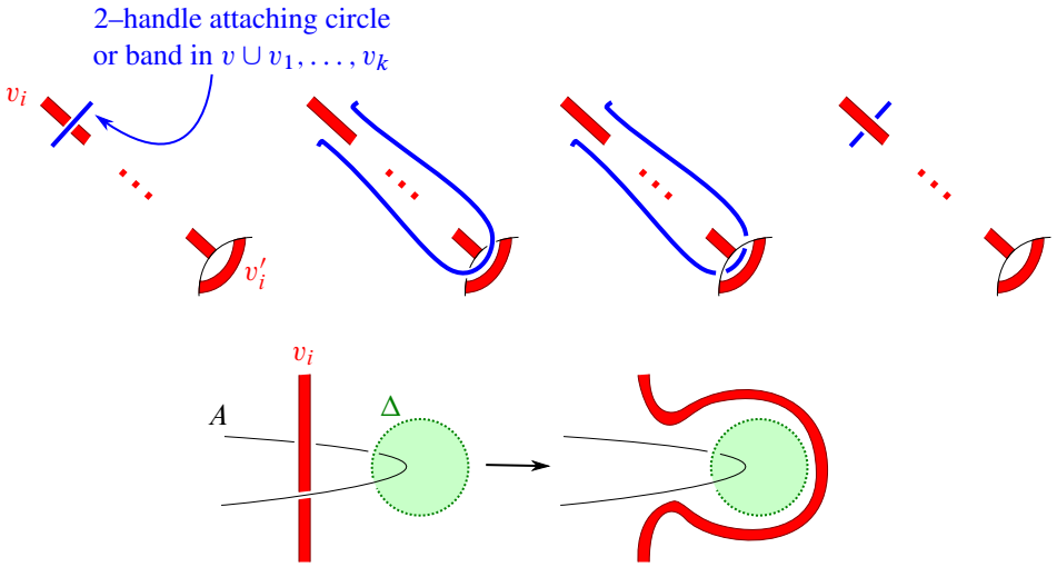
Figure 13: The proof of Theorem 6.16 : in a geometrically simply connected 4-manifold, two 0-concordant surfaces with simply connected complements are ambiently isotopic. Top: We may change crossings between \mathcal{K} and v_i or between v_j and v_i by band moves (and hence isotopy of F' ). Bottom: We may change crossings of v_i with L by sliding the core of the tube represented by v_i over an immersed 2-sphere dual to F' .
