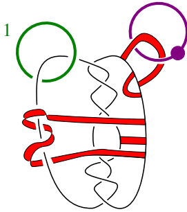
Figure 2: A banded unlink in Kirby diagram \mathcal{K} describing a torus \Sigma smoothly embedded in \mathbb{C}P^2 \# (S^1 \times S^3) . The 2-component unlink in E(\mathcal{K}) bounds two minima of \Sigma . Resolving the unlink along the four bands yields the boundary of two maxima of \Sigma . Then \chi(\Sigma) = 2 - 4 + 2 = 0 . One can check also that \Sigma is orientable.
